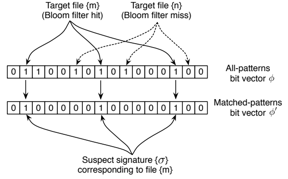
Figure 3: Building the matched-patterns bit vector as part of the feed-forward Bloom filter algorithm.
