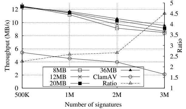
Figure 10: Performance for different size feed-forward Bloom filters, keeping the cache-resident portion constant.
